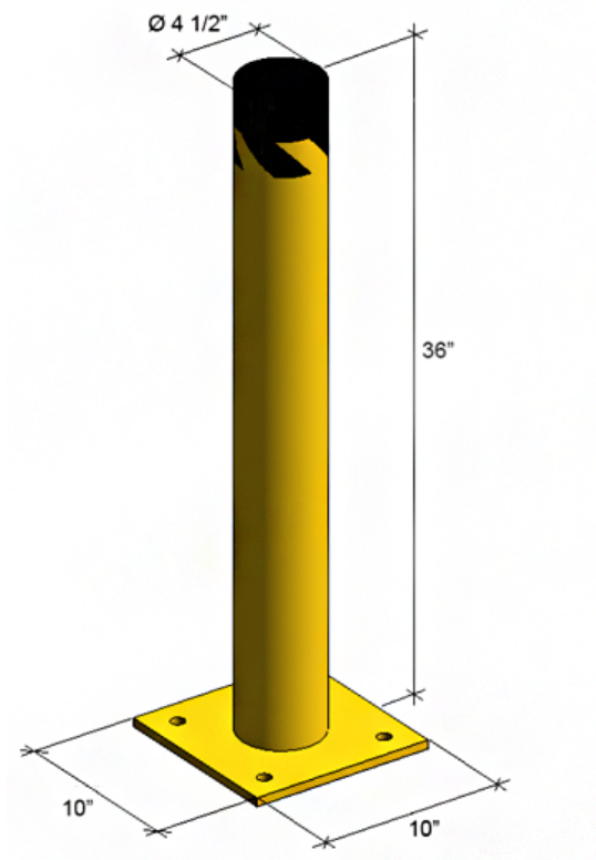
ITEM # B36 STANDARD HIGH BOLLARD HEIGHT 36"
